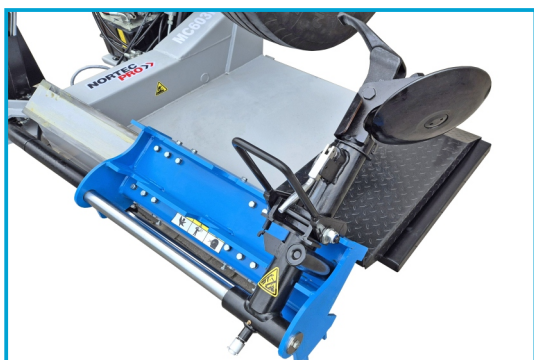
BRAKE AND CLAW ON A ROTATING HEAD
